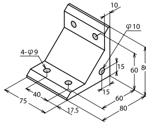
Model Number ABLH-8075-8
