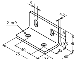
Model Number BLSM-4075-8
