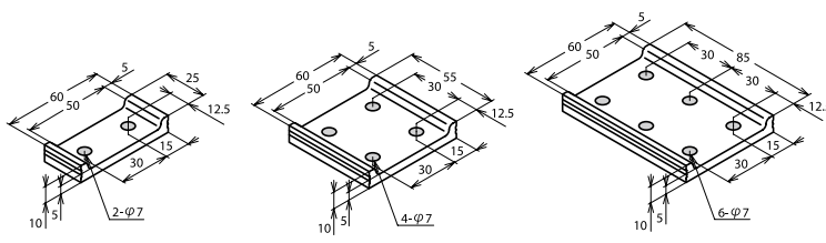
Model Number ABSP-6025-6
