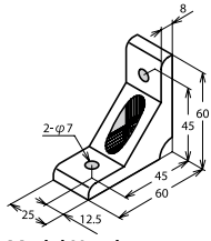
Model Number ABLR-6025-6
