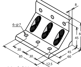
Model Number ABLR-6085-6
