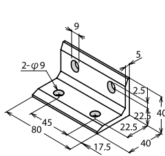
Model Number ABL-4080-8
