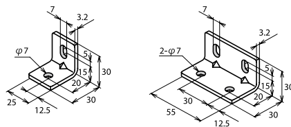
Model Number BLSM-3025-6
