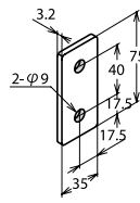
Model Number BPSM-3575-8
