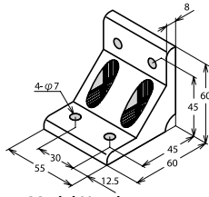
Model Number ABLR-6055-6
