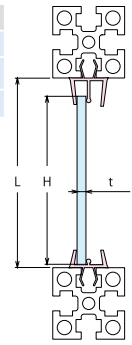
Cross-sectional view
