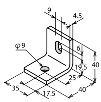
Model Number BLSM-4035-8
