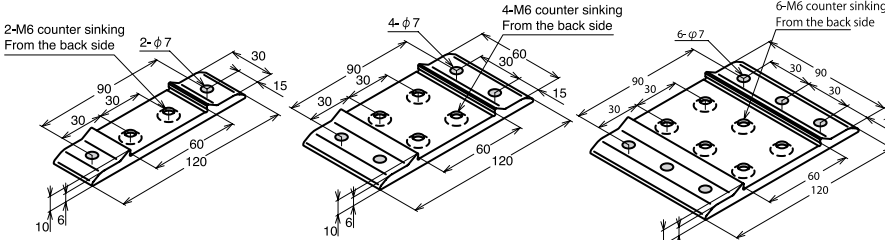
Model Number ABJF-6030-6
