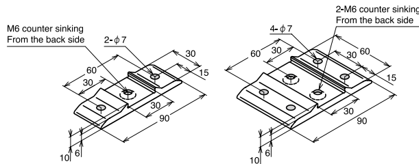
Model Number ABJF-3030-6
