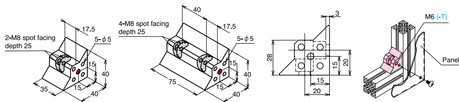
Model Number ABLB-4035-8(-T)
