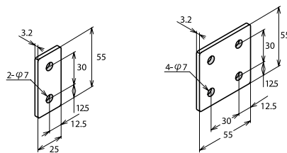
Model Number BPSM-2555-6
