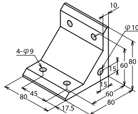
Model Number ABLH-8080-8
